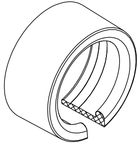
ISOMETRIC VIEW: CUT-AWAY TO SHOW PROFILE
