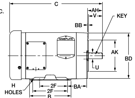
TEFC Enclosure
