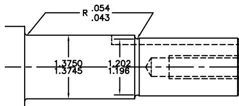
UNDERCUT DETAIL SCALE = .75
