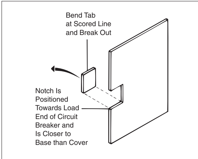
Figure 4 Scored Tab in Barrier.
