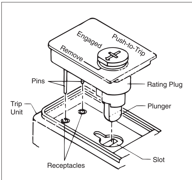
Figure 11 Installing Rating Plug.
