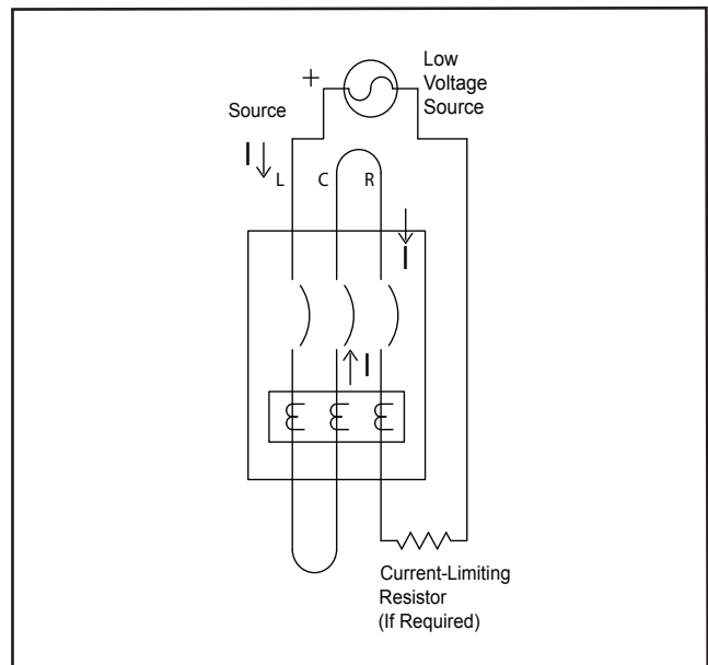
Figure 15-4b Connections for Ground Fault Trip Test with a Three-Wire System when testing the lowest GF pickup setting.
