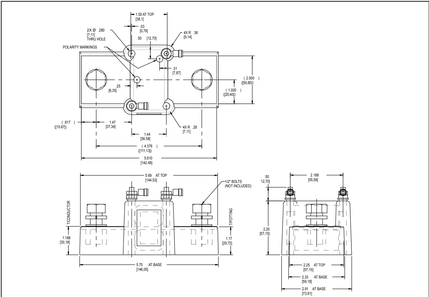
Figure 7 Neutral Current Sensor.
