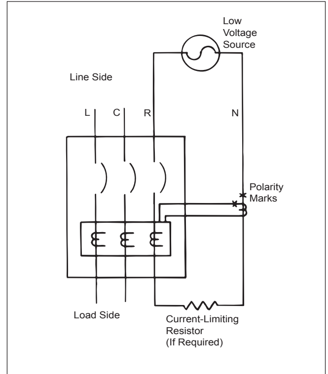
Figure 15-2 Connections for a No-Trip Test on Ground Fault for a Four-Wire System.
