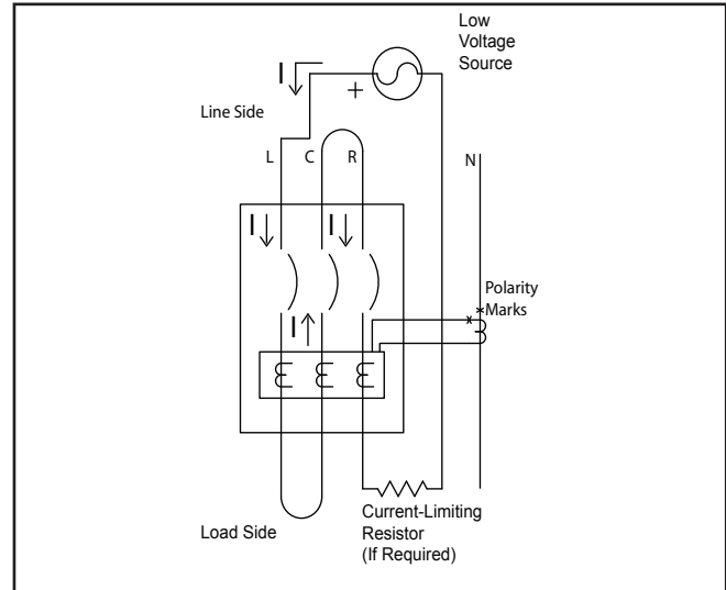
Figure 15-4a Connections for a Trip Test on Ground Fault when testing the lowest of pickup setting.
