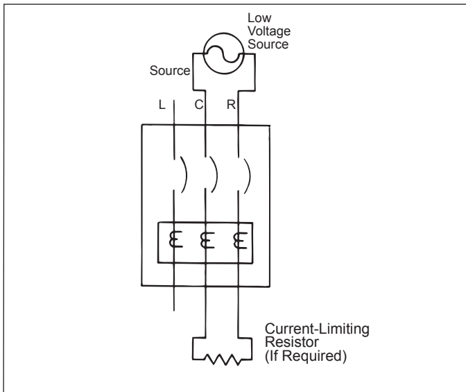
Figure 15-3 Connections for Ground Fault No-Trip Test with a Three-Wire System.
