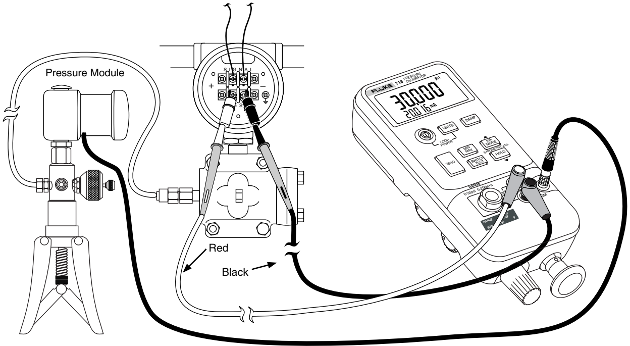
Figure 6. Pressure Module with External Pump
