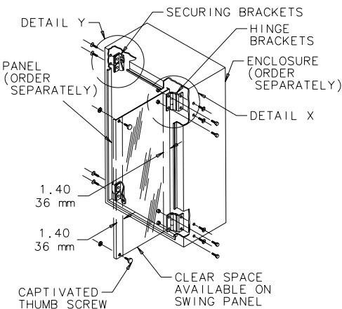
Wall-Mount Enclosure Swing-Out Panel Kit
