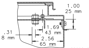
DETAIL X
