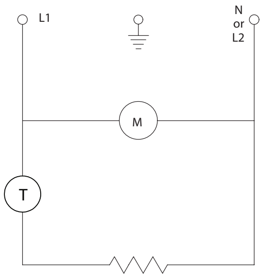
100-800 Watt Schematic
