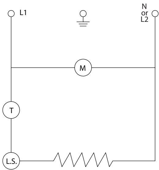
1300 Watt Schematic
