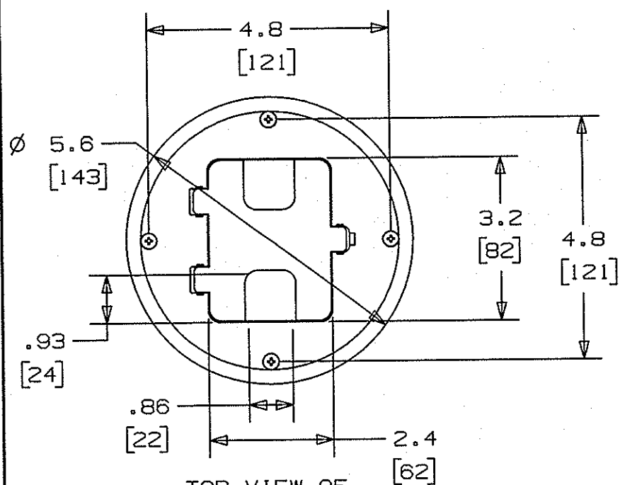
TOP VIEW OF CAT RF500XX
