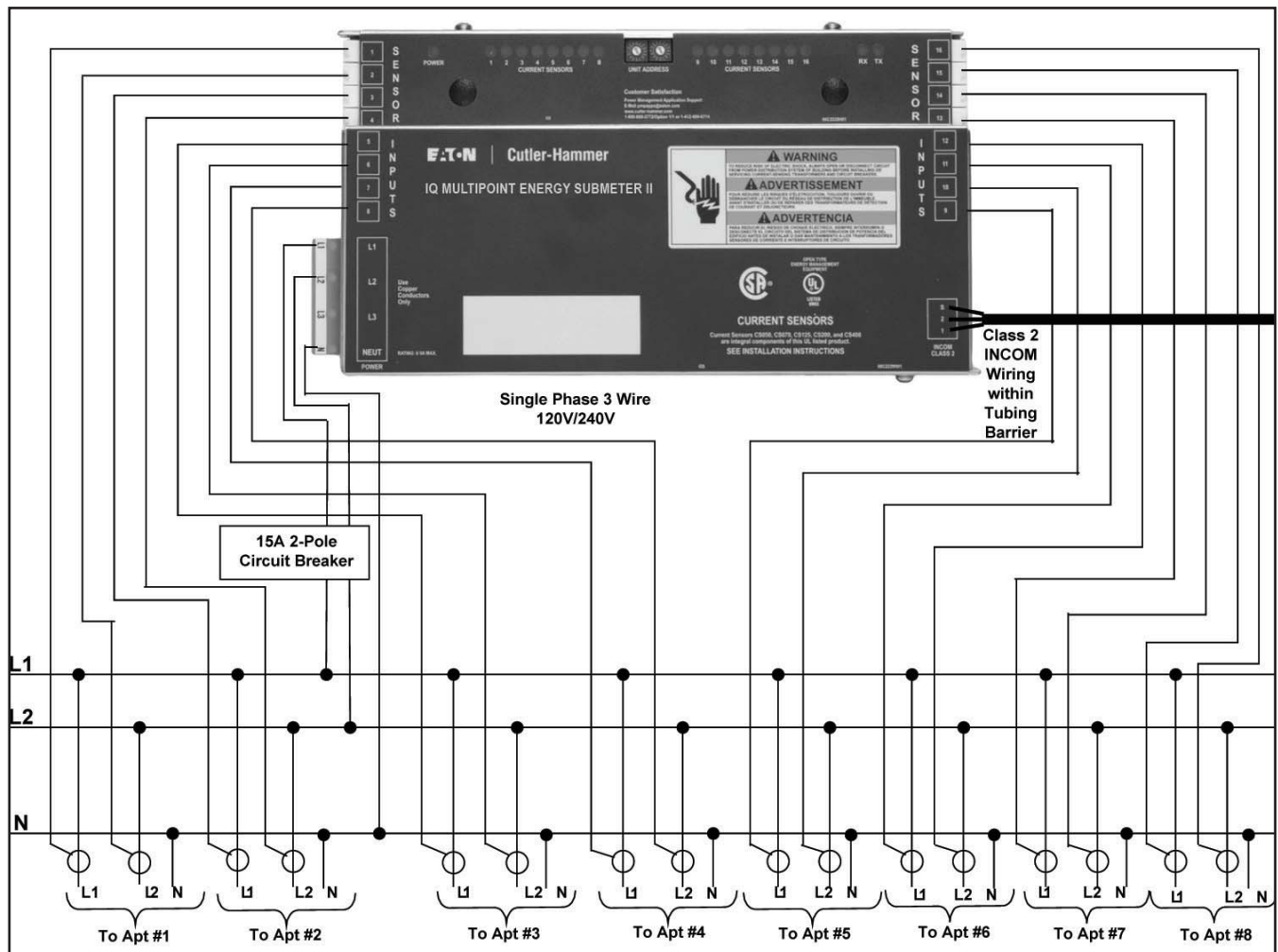
Figure 5.2 Example Wiring for Eight Two Pole Meter Points
