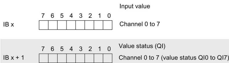
Figure 4-1 Address space of the DI 8x24VDC ST with value status
