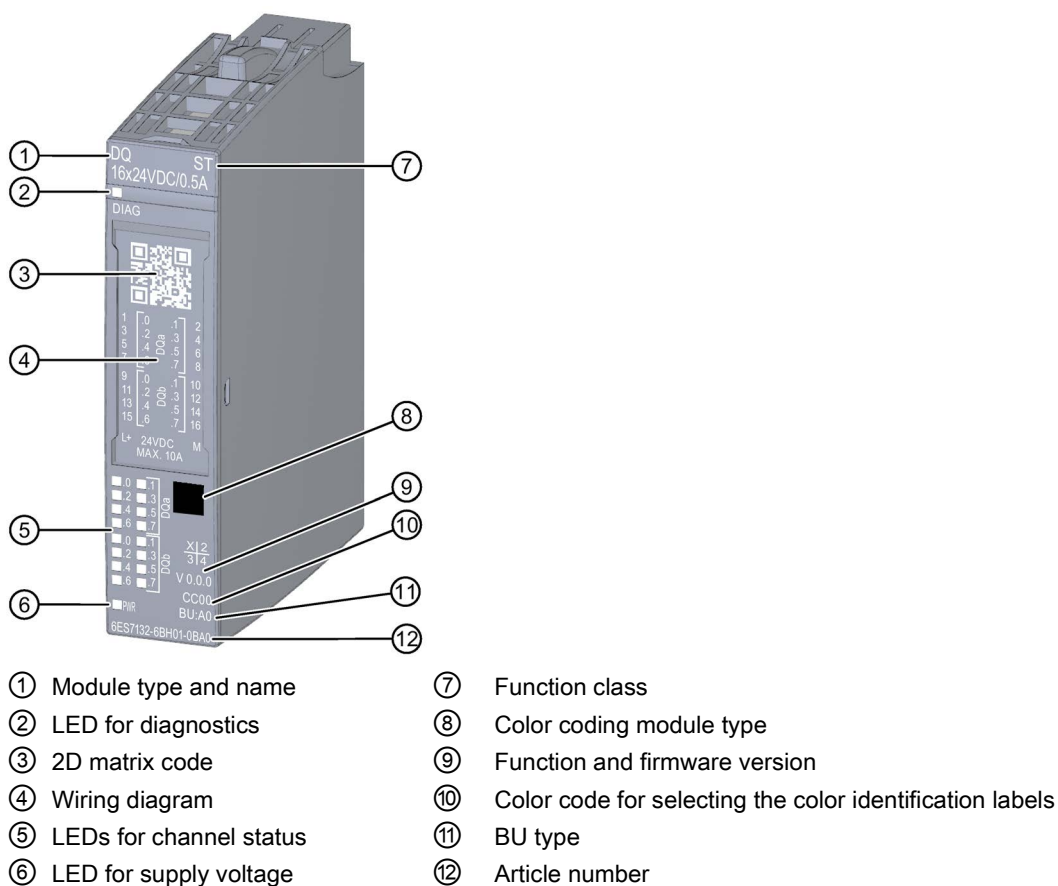
Figure 2-1 View of the module DQ 16x24VDC/0.5A ST
