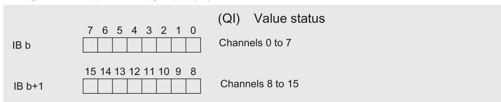
Figure 4-1 Address space of DQ 16x24VDC/0.5A ST with value status
