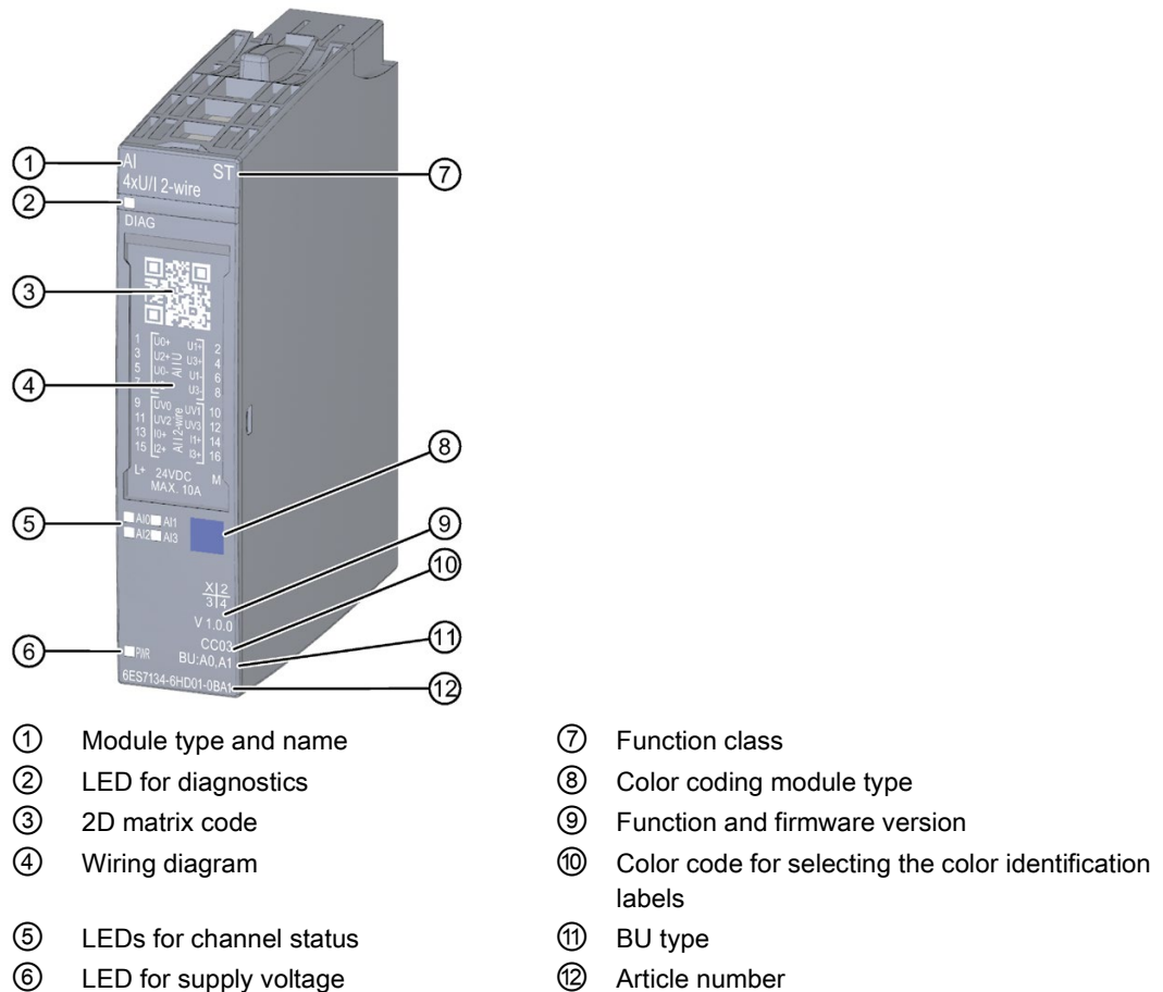
Figure 2-1 View of the module AI 4xU/I 2-wire ST
