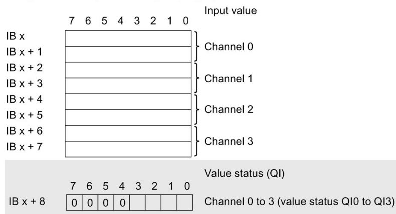
Figure 4-2 Address space of the AI 4×U/I 2-wire ST with value status
