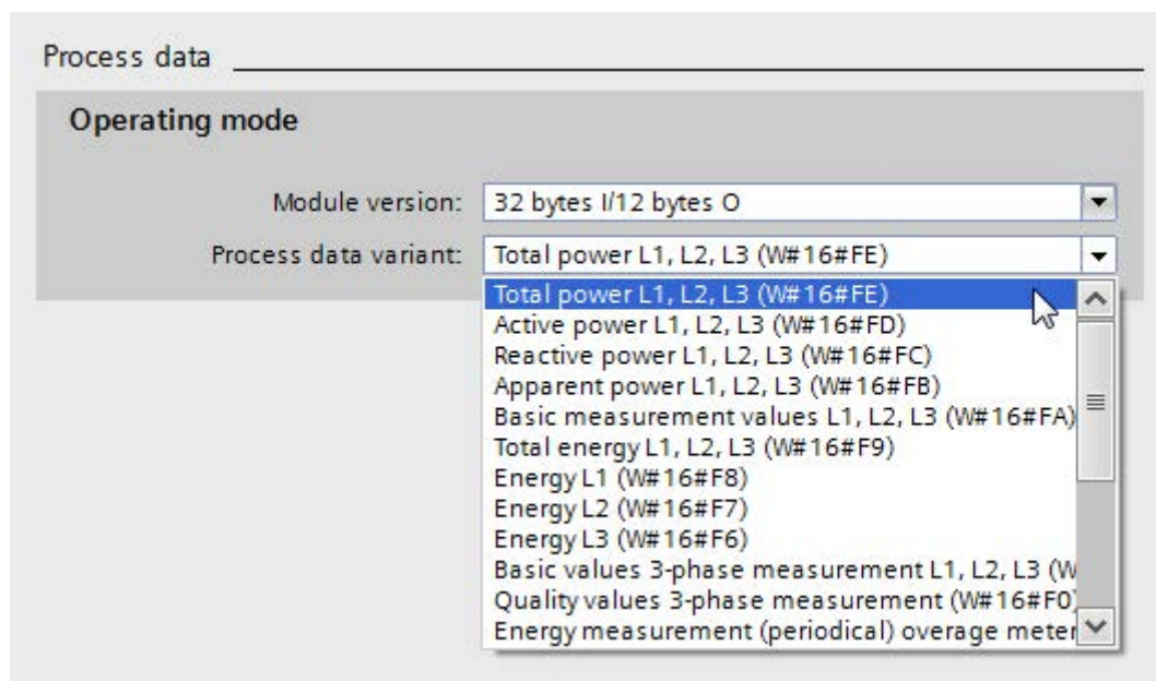
Image D-1 TIA Portal Process data variant device configuration
