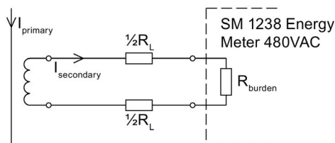
Image 3-2 Maximum length for connection cable
