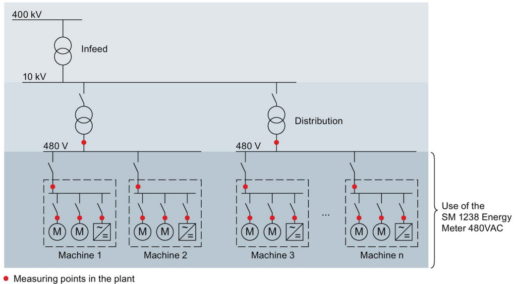
Image 2-1 Use of the SM 1238 Energy Meter 480VAC
