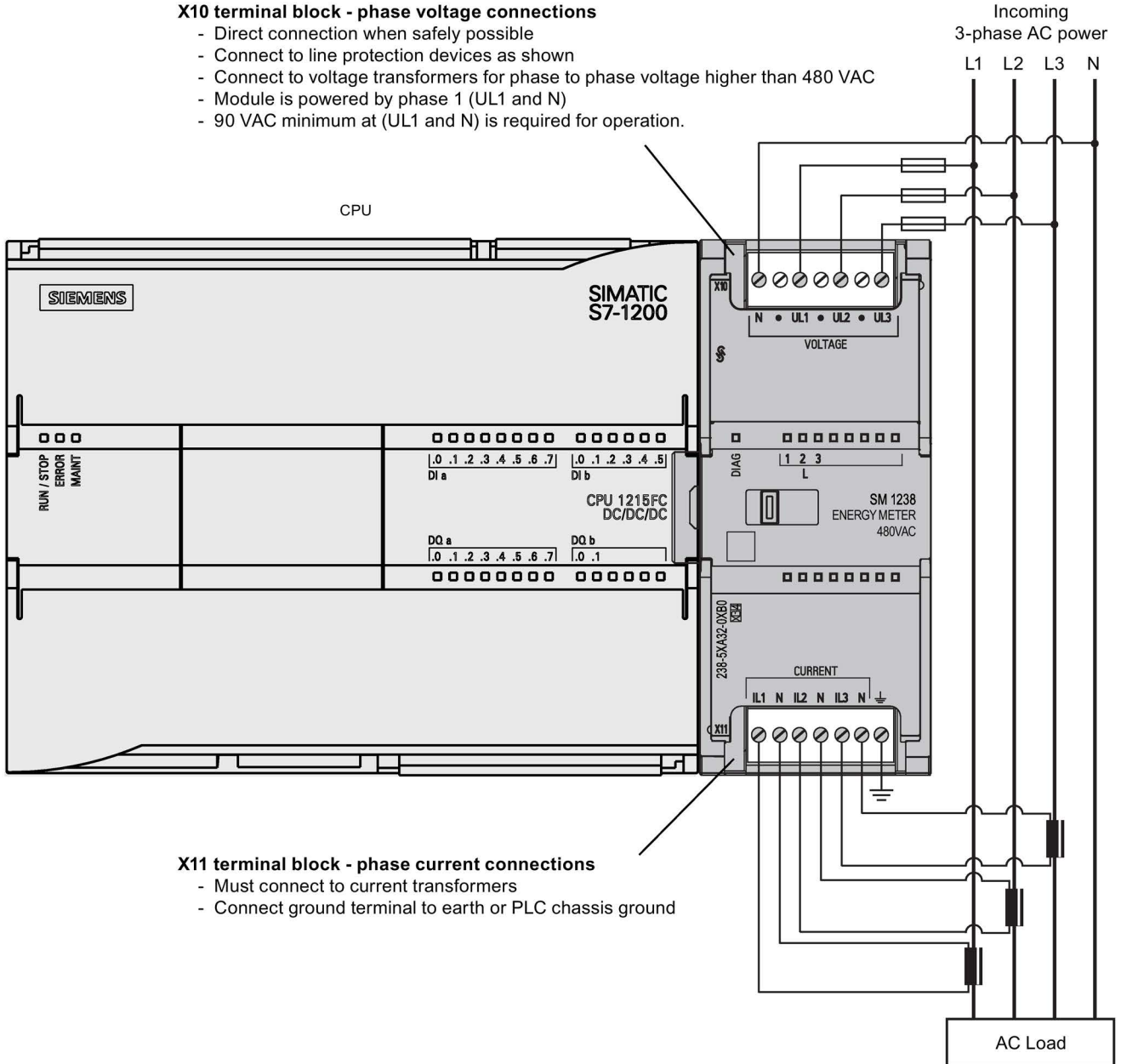
Image 3-1 SM 1238 Energy Meter 480VAC wiring diagram
