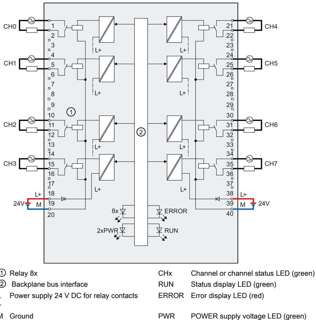
Figure 3-1 Block diagram and terminal assignment
