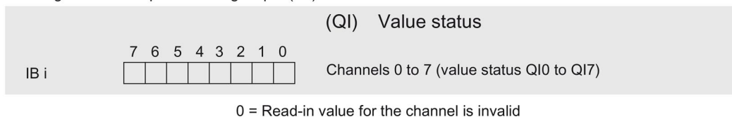
Figure 4-1 Address space for configuration as 8-channel DQ 8x230VAC/5A ST with value status
