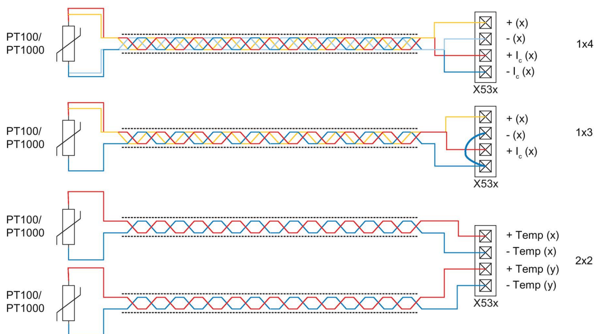
Figure 4-2 Connecting a PT100/PT1000 with 2x2, 3 and 4-wires to the temperature sensor inputs X53x of Terminal Module TM150
