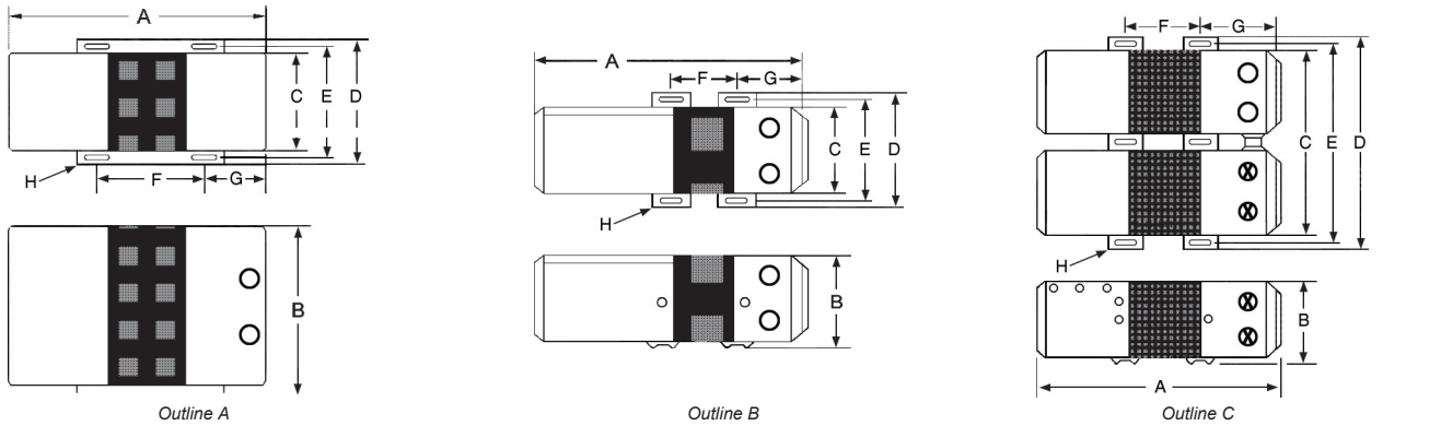
Figure 1: Mounting Holes and Dimensions
