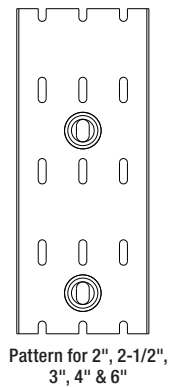
Bottom view
